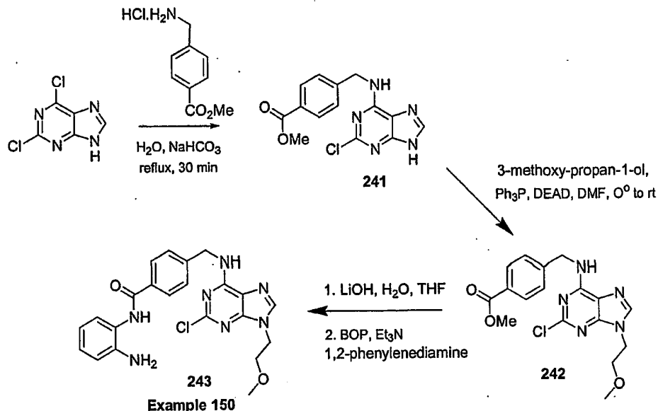
Scheme 39
